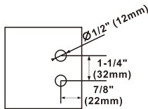
(LOCK CASE)
