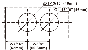
(LOCK BODY)
